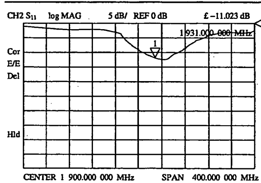
Return loss characteristic of the antenna in close proximity to the radio chassis (flip closed).
